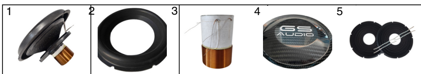
CUSTOMIZABLE COMPONENTS AND SPARE PARTS: 1. RECONE KIT - 2. SURROUND - 3. COIL - 4. DUSTCUP - 5. SPIDER PACK/SPIDER KIT
